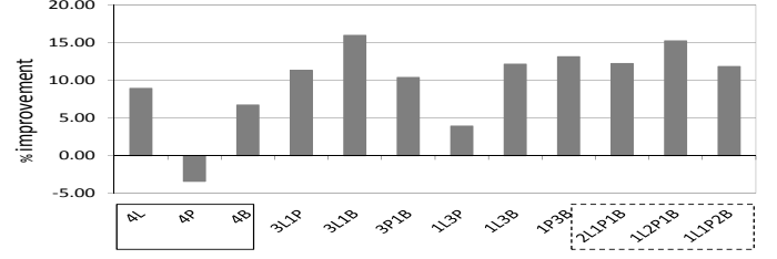
Fig. 5. Performance of heterogeneous memory system over DDR3 homogeneous memory for a 4-core system.
