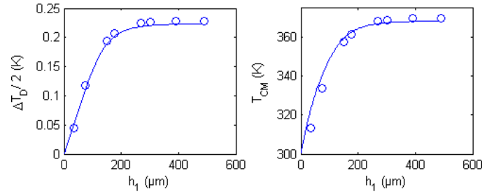
Figure 3. Differential temperature \Delta T_D/2 and common mode temperature T_{CM} vs. cavity depth (solid line: model, dots: FEM)
