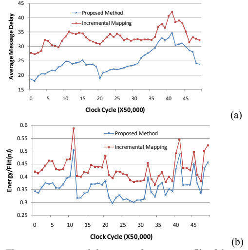
Figure 3. The average network latency and energy per flit of the proposed processor allocation and the incremental mapping.
