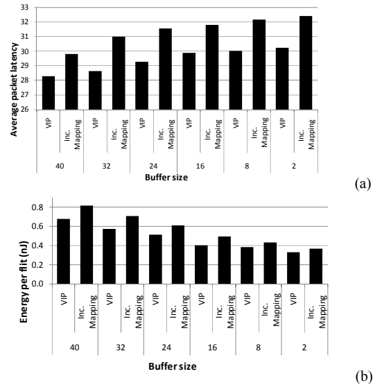
Figure 4. The average network latency (a) and energy per flit (b) of the proposed processor allocation and the incremental mapping for different buffer sizes.
