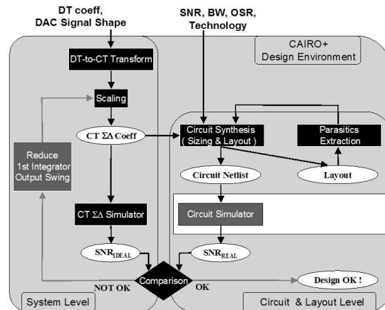
Figure 1. CT \Sigma\Delta modulator synthesis in the CAIRO+ design environment.
