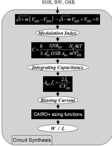
Figure 2. Integrator synthesis procedure.
