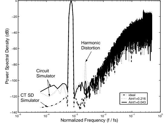
Figure 3. Comparison between ideal system-level \Sigma\Delta simulation & circuit level simulation.
