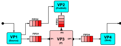
Figure 7: The LAURA hardware model of the DCT subnetwork.
