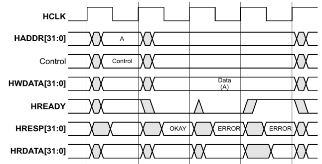
Figure 2: HREADY signal example
