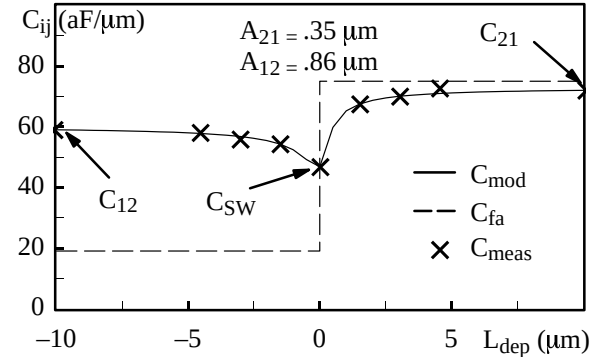
Figure 3: Fringing coefficient vs L_{dep} .
