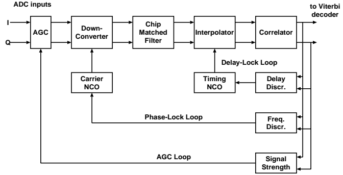
Figure 2: The SIMBA satellite receiver
