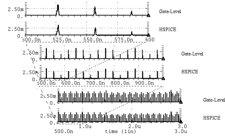
Figure 3. Gate level analysis versus SPICE
