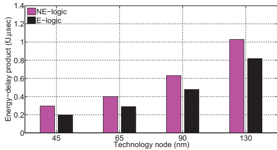
Fig. 8: Energy-delay product of a 8-bit carry lookahead adder designed using equalized logic (E-logic) vs. non-equalized logic (NE-logic) at zero word error rate at different technology nodes. The equalized logic approach reduces the energy-delay product of the sub-threshold logic by up to 26.46% across all technology nodes in the minimum energy supply voltage.
