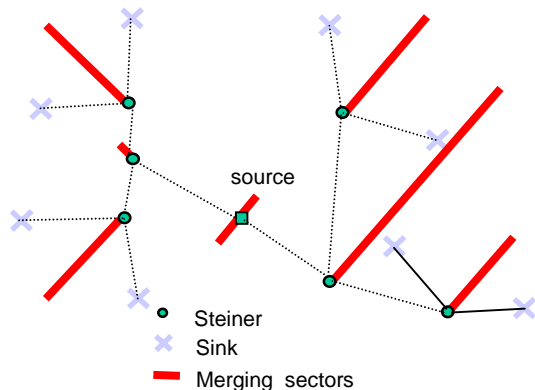
Figure 2: An example of bottom-up merging sequence
