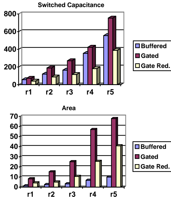
Figure 3: Comparison among different clock routing methods. Switched capacitance in pF, area in 10^6 \lambda
