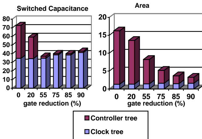
Figure 5: Gate reduction vs. switched capacitance and area for benchmark r1
