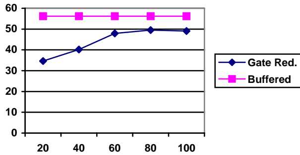
Figure 4: Average module activity (x-axis) vs. switched capacitance (y-axis) for benchmark r1
