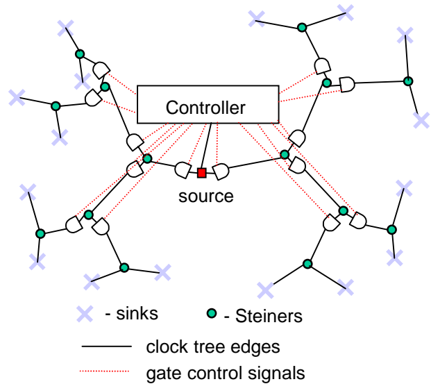
Figure 1: Gated clock tree
