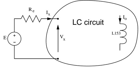
Figure 1: The PEEC circuit
