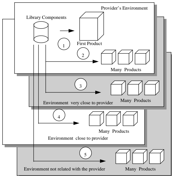
Figure 1.- Reusability Levels.
