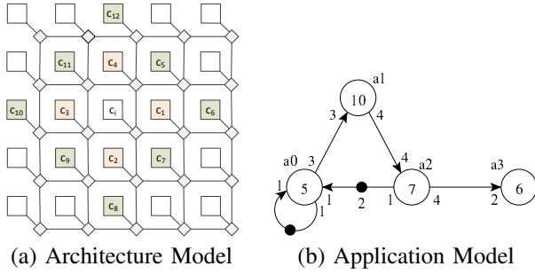
Fig. 1. Application and architecture example II. RELATED WORKS
