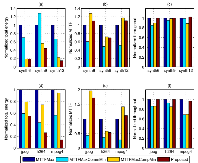
Fig. 6. Temperature-reliability-performance trade-offs
