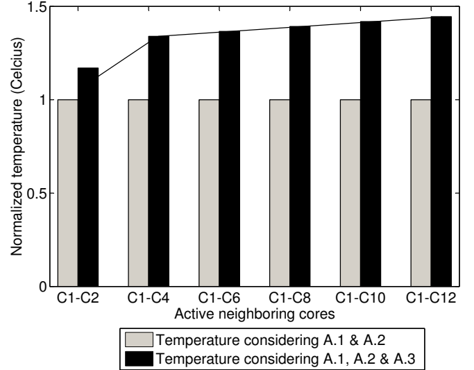
Fig. 2. Temperature underestimation by ignoring component A.3. The level C1 - Cn indicates cores c_1, c_2, \dots, c_n active simultaneously.
