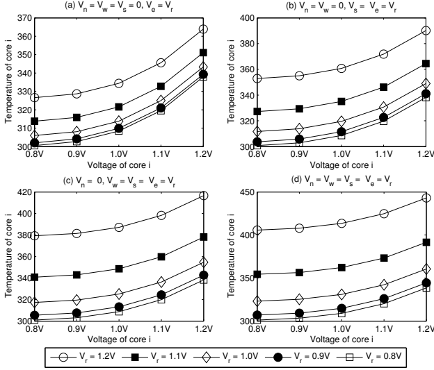
Fig. 3. Temperature (in Kelvin) Characterization
