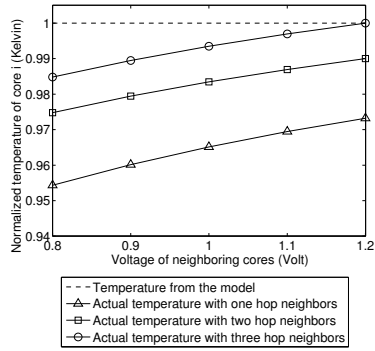
Fig. 4. Temperature variation of the proposed model
