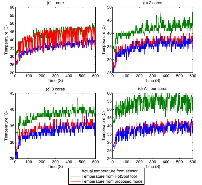
Fig. 5. Validation of the proposed model – MPEG 4 case study
