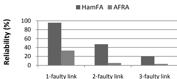
Fig. 4. Reliability analysis
