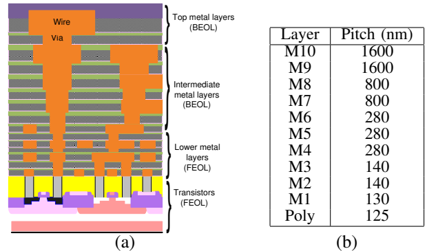
Fig. 1: (a) A cross-section of an IC layout. The layout has two parts: Front End Of Line or FEOL layers (transistors, lower metal layers) and Back End Of Line or BEOL layers (intermediate, and top metal layers) [Source: [10]]. (b) Pitch length of different metal layers in 45nm CMOS technology [1].
