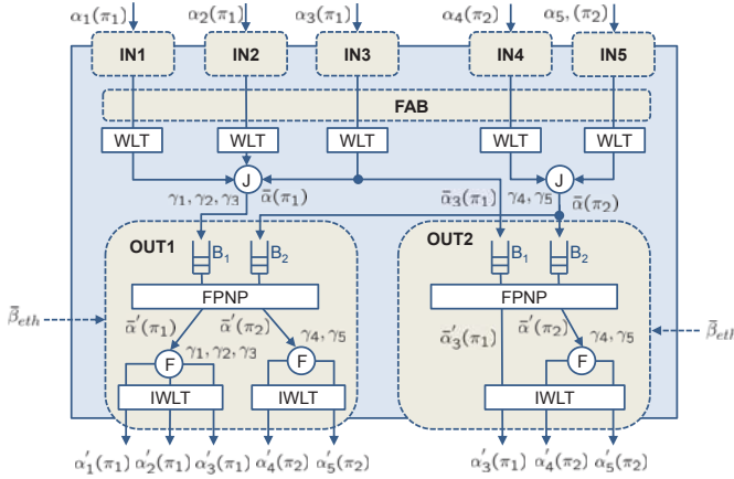
Fig. 5. This figure shows the data path of streams in a switch model.
