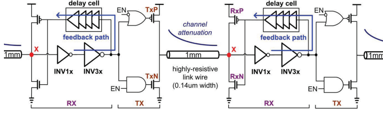
Fig. 2: Proposed clockless low-swing voltage-locked repeater (VLR) for single-cycle multi-hop link traversal.
