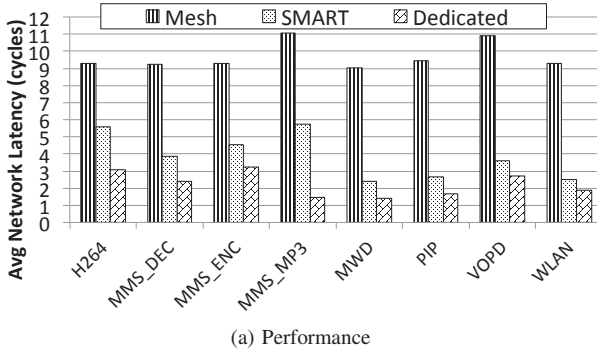
Fig. 10: Evaluation of SMART NoC across SoC Applications.
