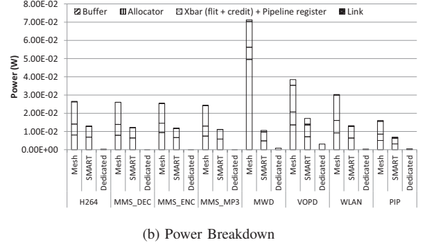
Fig. 10: Evaluation of SMART NoC across SoC Applications.
