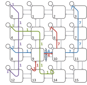
Fig. 7: SMART NoC in action with four flows. (The number next to each arrow indicates the traversal time of that flow.)
