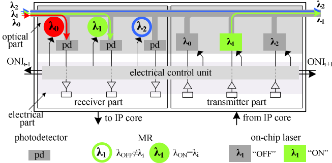
Figure 2: Optical Network Interface
