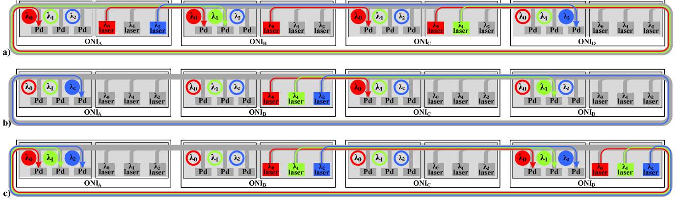
Figure 3: Possible communication schemes: a) dedicated distributed point to point communications channel, b) broadcast and c) high bandwidth channel
