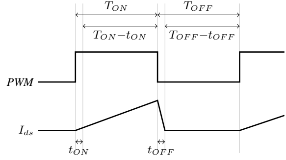
Fig. 4: Illustration of the ON and OFF phases of a PWM pulse with the respective delays for t_{ON} and t_{OFF} of the drain-source current I_{ds} of a MOSFET switched by the PWM signal.
