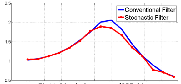
Fig.11a Magnitude response of LPF_2A
