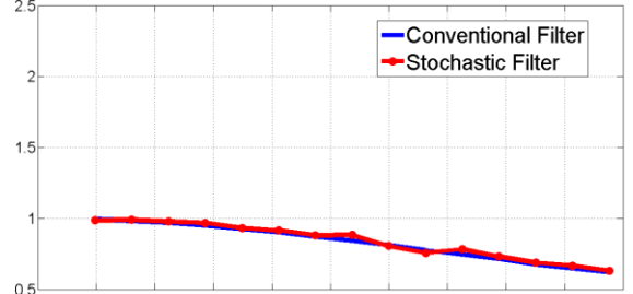
Fig.11b Magnitude response of LPF_2B
