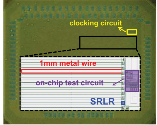
Fig. 7. Die photograph of the test chip in 45nm SOI CMOS.
