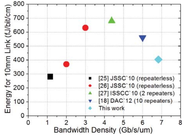
Fig. 8. 1cm LT energy versus bandwidth density of the proposed on-chip signaling and previous works.
