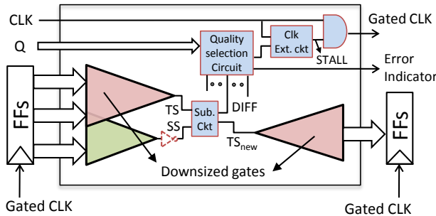
Fig. 2: Quality configurable circuit design using SASIMI
