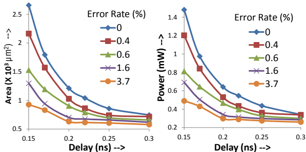
Fig. 6: Area and power of KSA with delay sweep
