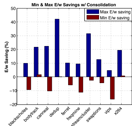
Fig. 1: Minimum and maximum change in E/w when a PARSEC application is consolidated with another PARSEC benchmark on an AMD Magny-cours server, each running with 6 threads, w.r.t. running the benchmarks separately with 12 threads.
